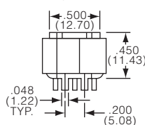
Double pole
