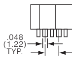
Single pole
